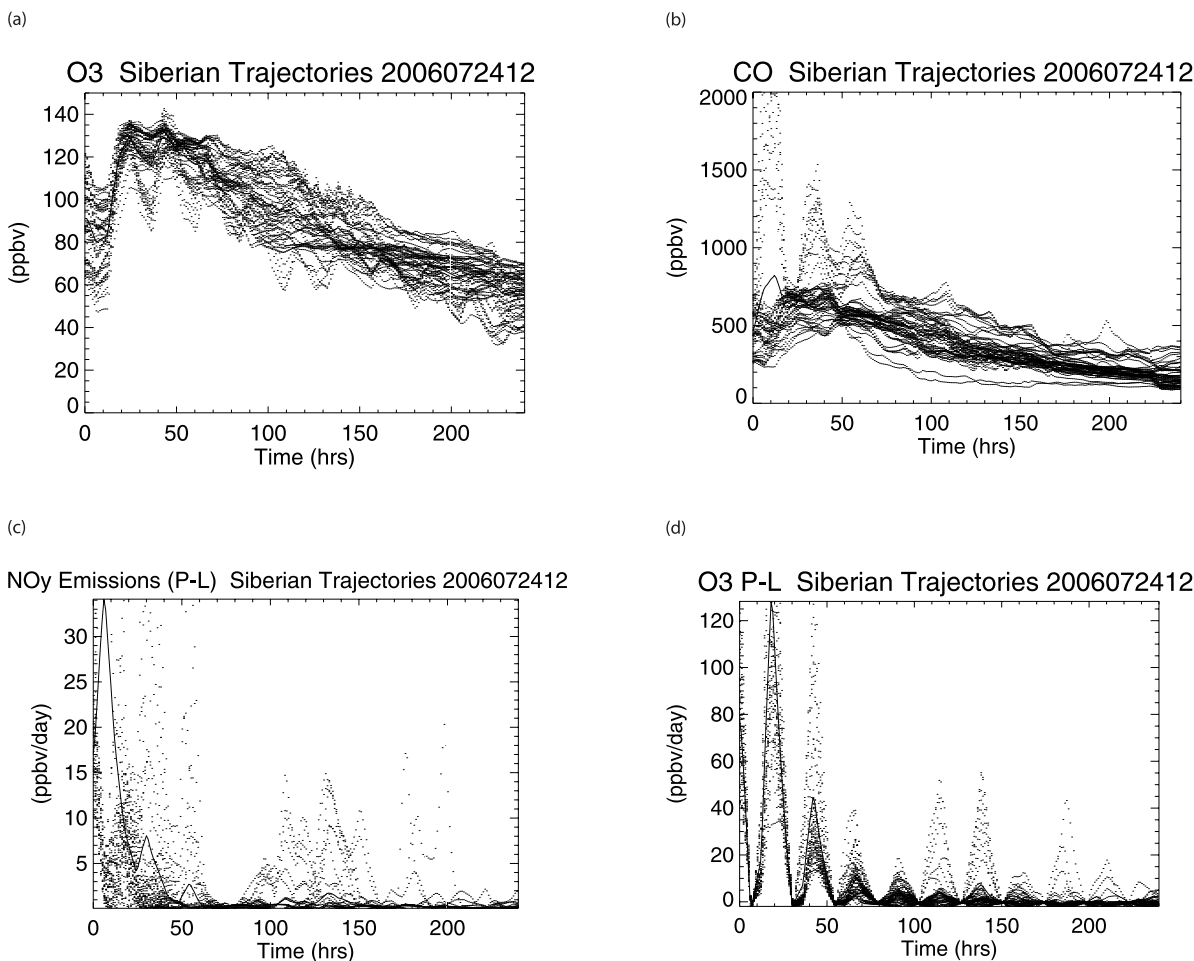
Figure 8. The 10-day forward trajectory simulation without aerosols initialized with 24 July 2006 upwind data and daily fire emissions (Tg/day) from real time MODIS fire counts at Siberia showing time evolution of (a) O 3 concentrations, (b) CO concentrations, (c) NO y , and (d) O 3 production rates.
