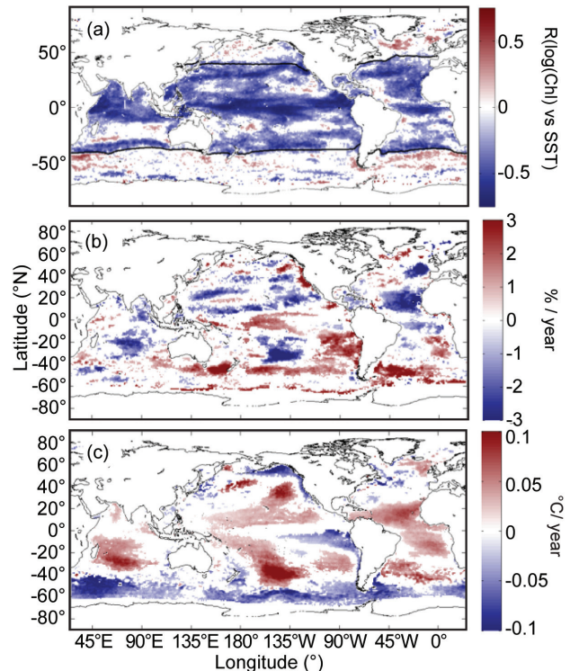
FIG. 3.38. (a) Spatial distribution of the local-scale correlation coefficient ( R ) between \ln(\text{Chl}) and SST, (b) local-scale time trends in \ln(\text{Chl}) anomalies (in % \text{yr}^{-1} ), and (c) local-scale time trends in SST anomalies (in ^{\circ}\text{C} \text{yr}^{-1} ). Only significant (95% confidence interval) correlations and trends are plotted. Calculations are made over the entire SeaWiFS record (Oct 1997–Dec 2010) and on a local-scale 1° bin in latitude and longitude. Also shown in (a) is the 15°C SST isotherm (black line).
