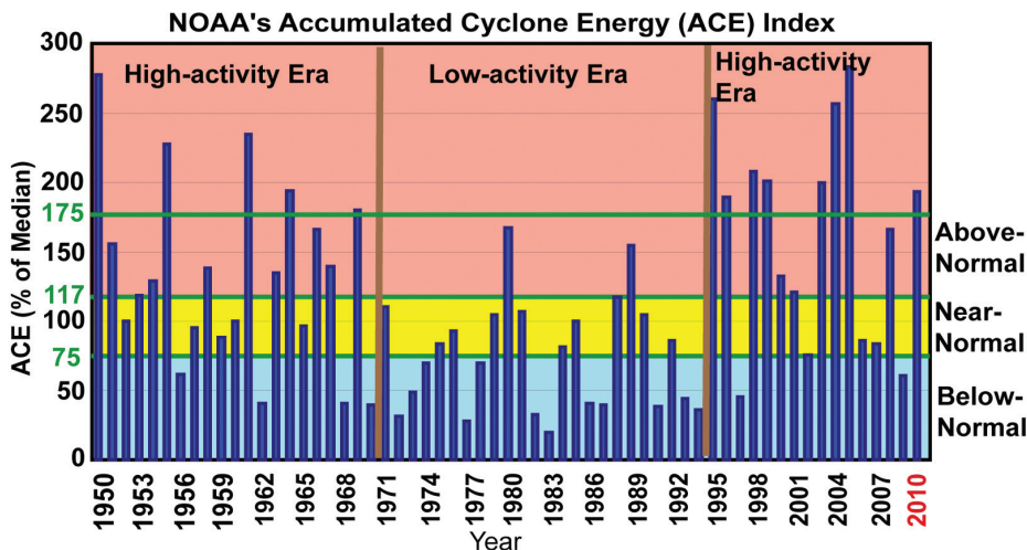
FIG. 4.9. NOAA's Accumulated Cyclone Energy (ACE) Index in the Atlantic Basin expressed as percent of the 1950–2000 median value ( 87.5 \times 10^4 \text{ kt}^2 ). The ACE is a wind energy index that measures the combined strength and duration of the named storms. ACE is calculated by summing the squares of the six-hourly maximum sustained wind speed (measured in knots) for all periods while the named storm has at least tropical storm strength. Pink, yellow, and blue shadings correspond to NOAA's classifications for above-, near- and below-normal seasons, respectively. The 175% threshold for a hyperactive season is indicated. Vertical brown lines separate high-activity and low-activity eras.
