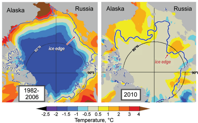
FIG. 5.5. Summer (June–September) SST anomalies in 2010 (right panel) relative to the summer mean during 1982–2006 (left panel). The anomalies are derived from satellite data according to Reynolds et al. (2002). The September mean ice edge (thick blue line) is also shown.
