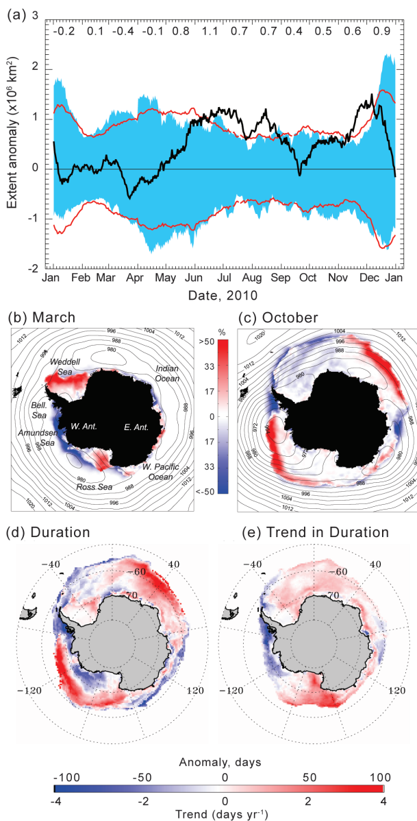
FIG. 6.7. (a) Plot of daily anomaly (black line) from the climatology (1979–2008) of daily Southern Hemisphere sea ice extent for 2010, based on satellite passive microwave ice concentration data from the GSFC Bootstrap Version 2 dataset (Comiso 1999, updated 2008). Blue banding represents the range of daily values for 1979–2008, while the red line represents \pm 2 standard deviations. At the top are monthly-mean extent anomalies ( \times 10^6 km 2 ). (b–c) Sea ice concentration anomaly maps for March and October 2010 derived versus the monthly means for 1979–2007, with monthly-mean contours of MSLP [from the Australian Community Climate and Earth System Simulator (ACCESS)] provided by the Australian Bureau of Meteorology. (d) Sea ice duration anomaly for 2010/11, and (e) duration trend. For (d) and (e), see Stammerjohn et al. (2008) for a description of techniques (using daily satellite passive-microwave data). Both the climatology (for computing the anomaly) and trend are based on 1979/80–2007/08 data, for which GSFC Bootstrap Version 2.0 data were available (Comiso 1999, updated 2008), while the 2010/11 duration-year data are from the NASA Team Near-Real-Time Sea Ice (NRTSI) dataset (Maslanik and Stroeve, 1999). The 2010/11 duration anomaly is therefore the 2010/11 NRTSI data minus the 1979/80–2007/08 BS V2 Climatology. Discrepancies introduced by using these different data sources lead to an uncertainty (difference) level that is well below the magnitude of the large changes/anomalies.
