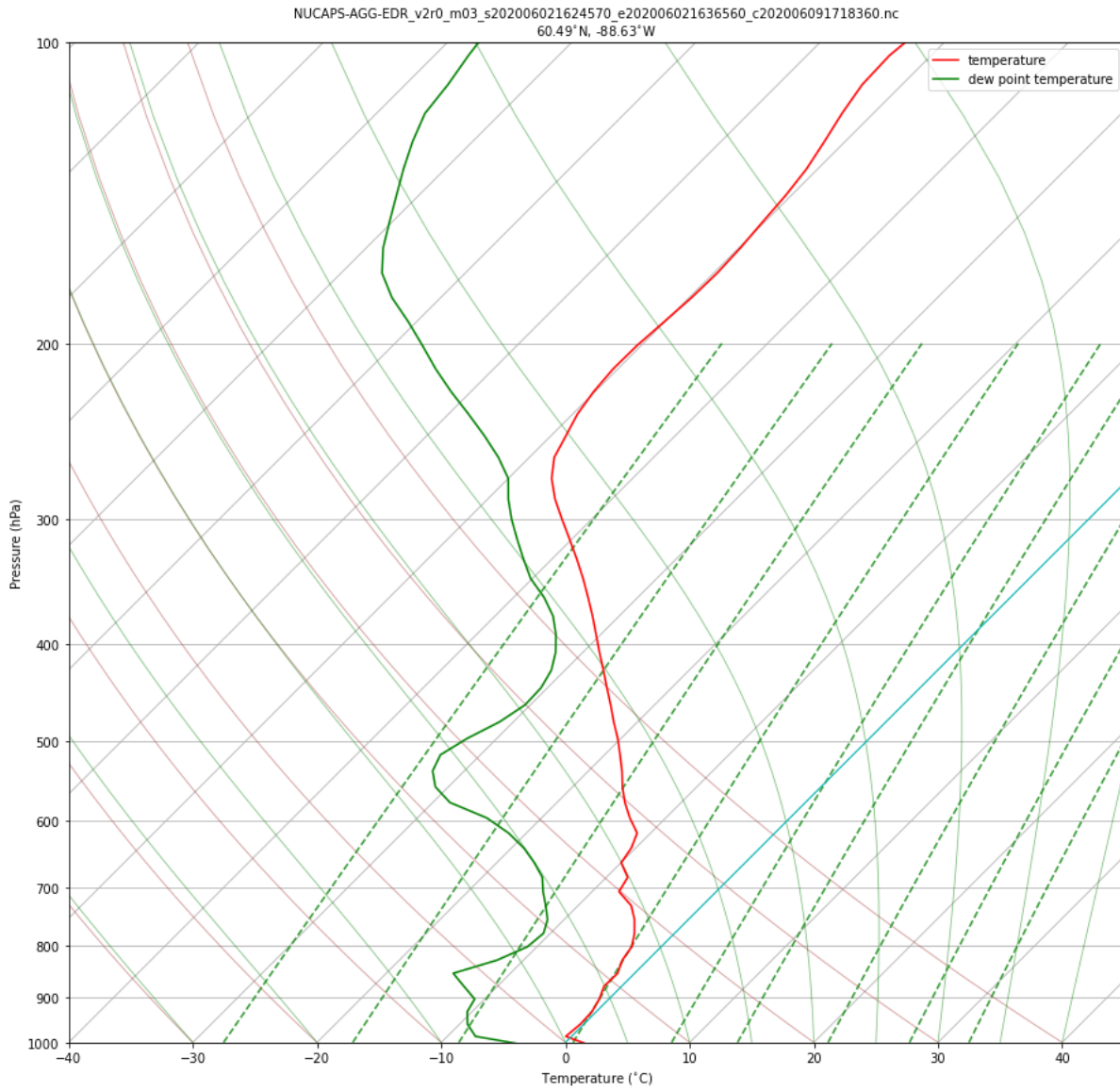
Figure 2: Skew-T diagram created from the CSPP_HEAP test output NUCAPS-AGG-EDR retrieval for 2 June 2020.
