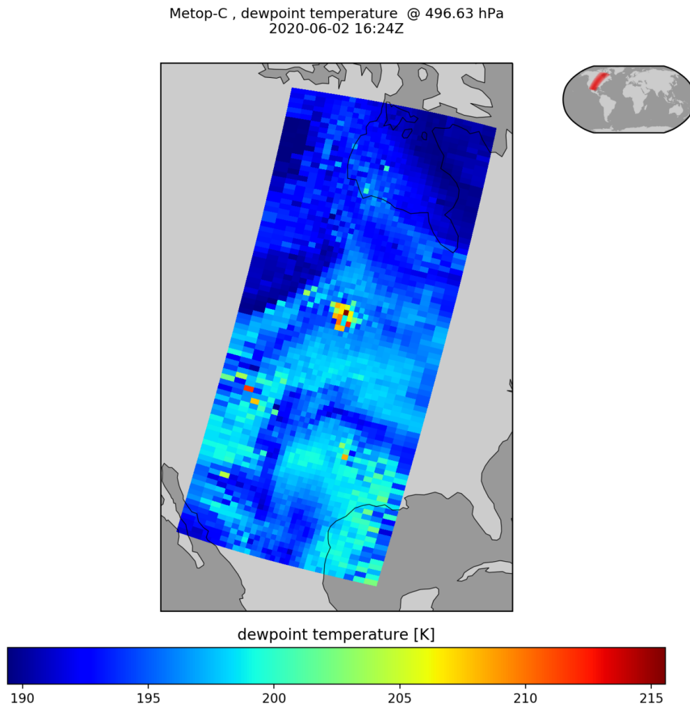
Figure 1: 496 hPa dew point temperature plot created from CSPP_HEAP retrievals from Metop-C (m03) on 2 June 2020.
