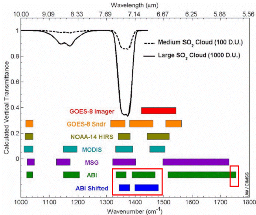
Figure 4. Spectral widths of several spectral bands near the SO 2 signature (from F. Prata of (CSIRO)).
