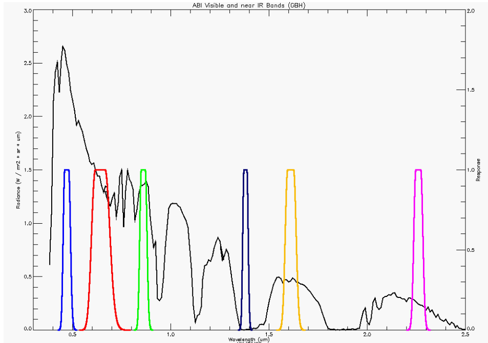
Figure 1. The spectral coverage of the six visible/near infrared bands with a representative clear-sky radiance plot.
